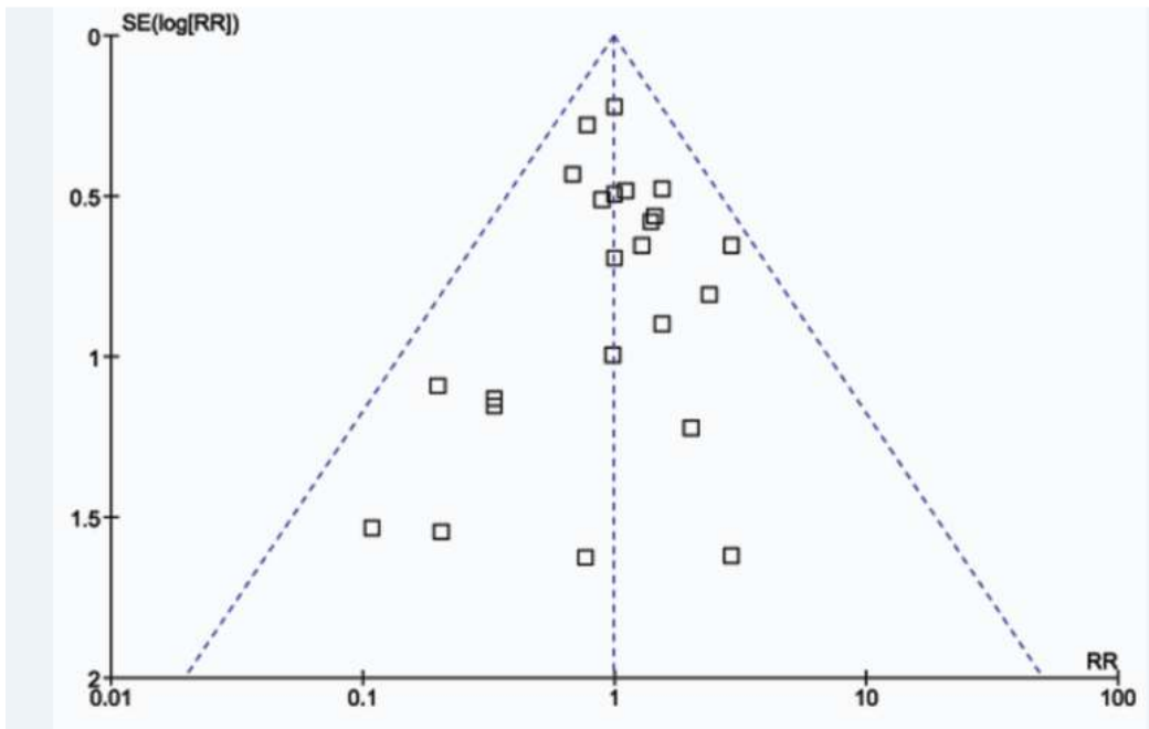
Fig. 2. Funnel plot of meta-analysis
