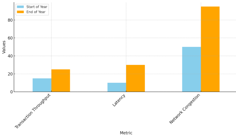
Fig. 8. Start vs End of Year Metrics
