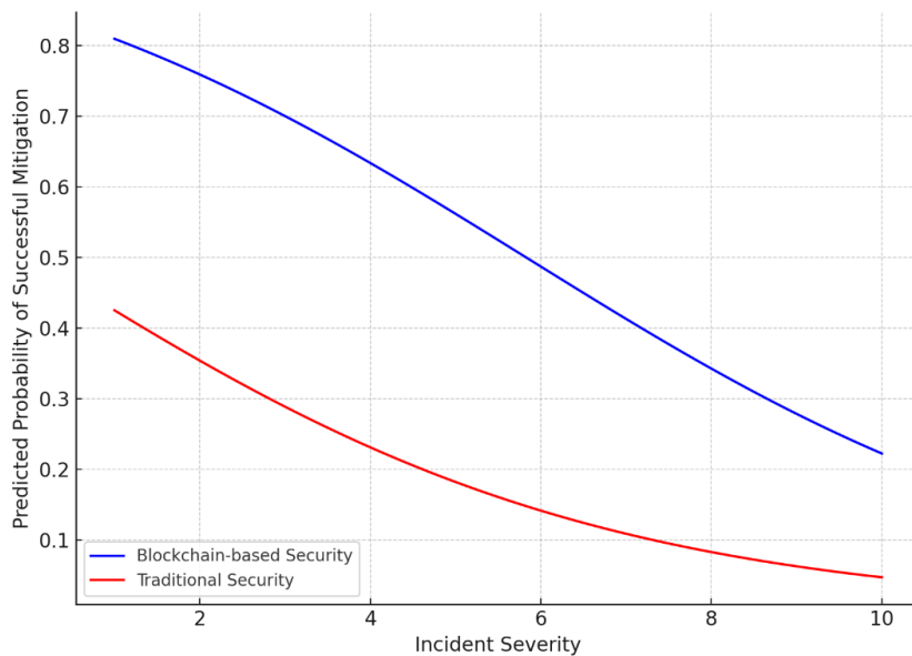
Fig. 5. Predicted probability of mitigation success by security measure
