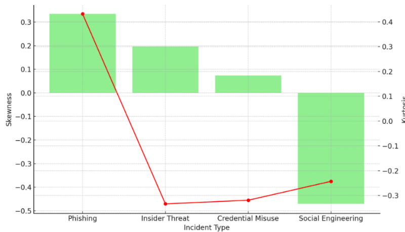
Fig. 2. Skewness and Kurtosis by Incident Type
