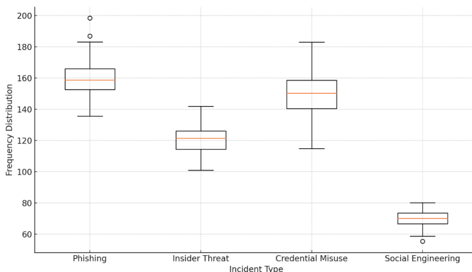
Fig. 1. Distribution of Incident Frequencies Across Vulnerability Types 2. Skewness and Kurtosis by Incident Type
