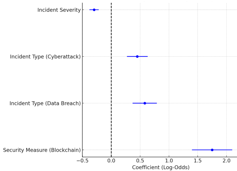
Fig. 4. Coefficient plot (Log-Odds) for logistic regression
