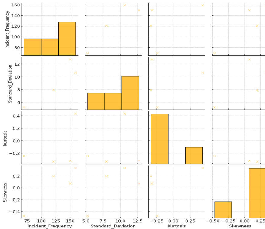
Fig. 3. Pair plot of Incident Statistics
