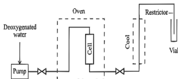
Fig. 6. Schematic diagram of the superheated water extraction apparatus
