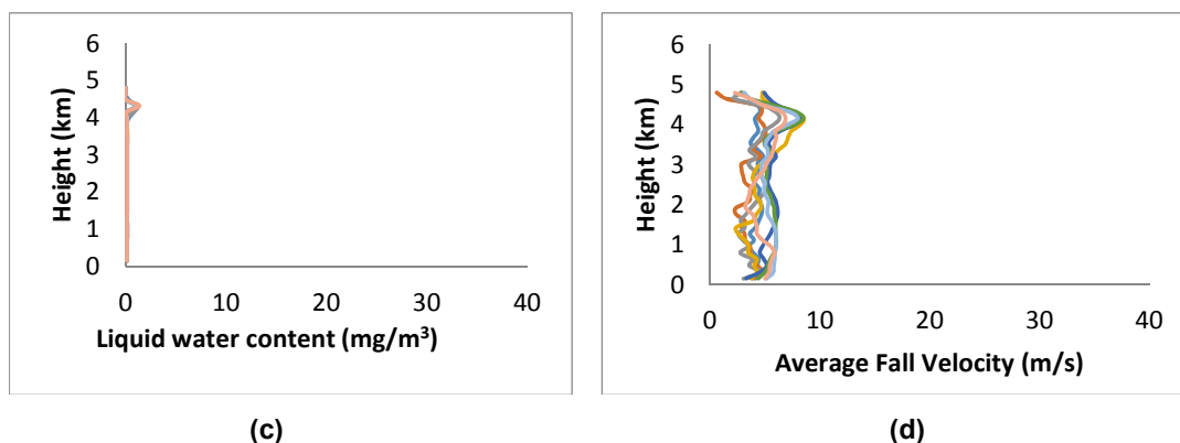
Fig. 4. Vertical profiles spectrum of different rain parameters obtained by MRR showing the Bright Band (BB) regions of rain event at 16:20-16:30 GMT LT on 26th October 2010 (a) Radar reflectivity profile (b) rain rate (c) Liquid water content, and (d) average fall velocity
