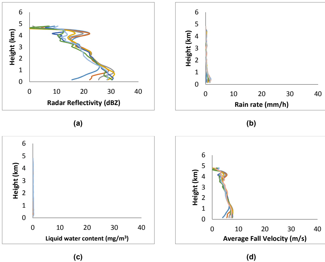
Fig. 3. Vertical profiles spectrum of different rain parameters obtained by MRR showing no Bright Band (NBB) regions of rain event at 16:55-17:20 GMT LT on 26th October 2010 (a) Radar reflectivity profile (b) rain rate (c) Liquid water content, and (d) average fall velocity
