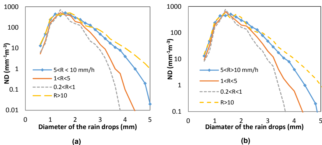
Fig. 5. A typical DSD measured on 26th October 2010 at (a) 160 m (16:20:15 LT) and (b) 640 m (17:10:15LT for different rain events
