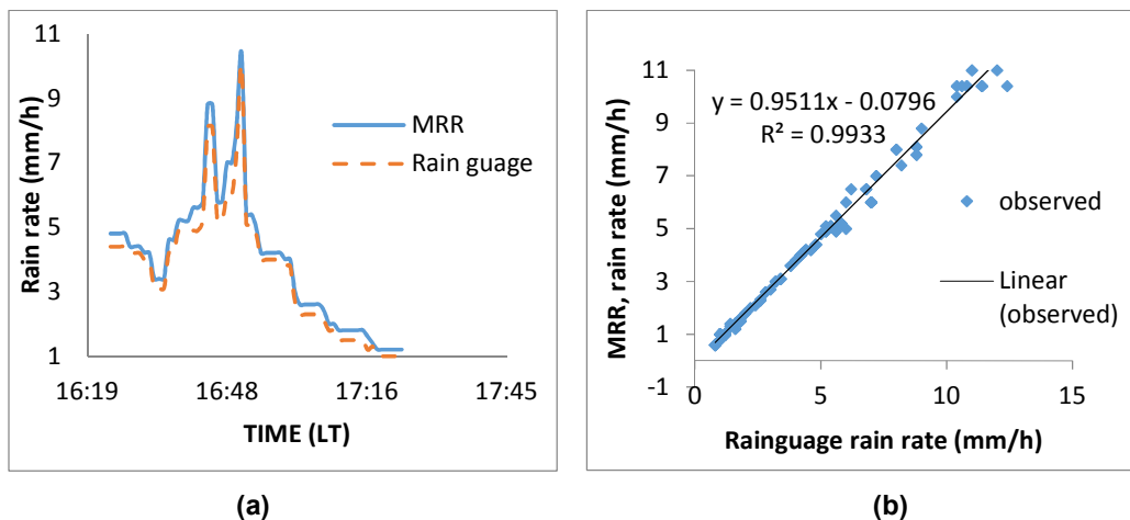
Fig. 6. (a) Comparisons of rain rates (b) Scattered plots of MRR rain event with rain gauge measurements as observed on the 26th October 2010
