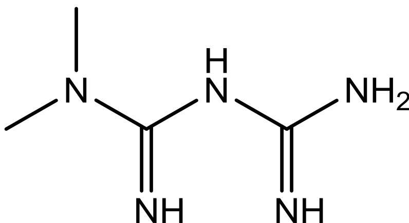
Fig. 10. Structure of metformin
