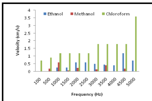
Fig. 6. Effect of PWM on fluid velocity at 500 C
