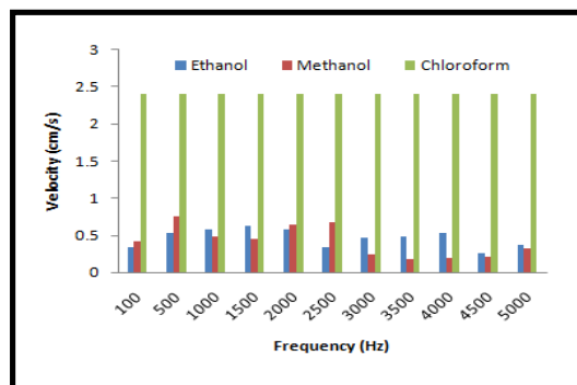
Fig. 7. Velocity plot for different fluids flowing across micro-channel at different frequencies
