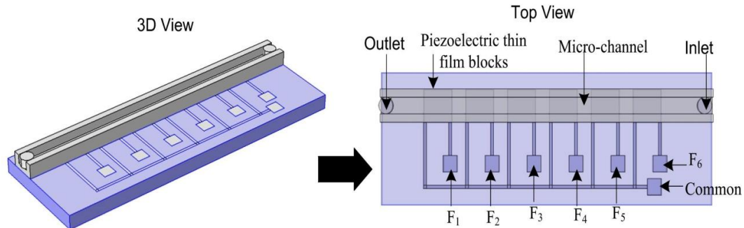
Fig. 8. Schematic showing different frequencies applied to microfluidic channel
