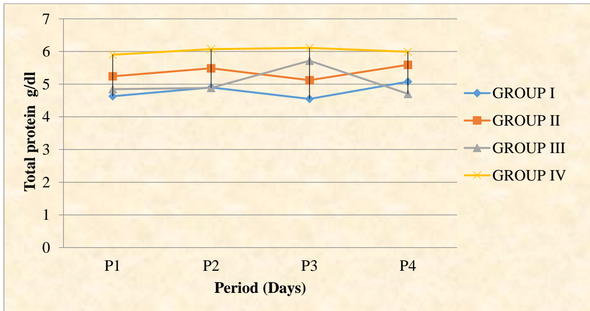
Fig. 1. Total protein levels (g/dl) at various periods in different treatment groups
