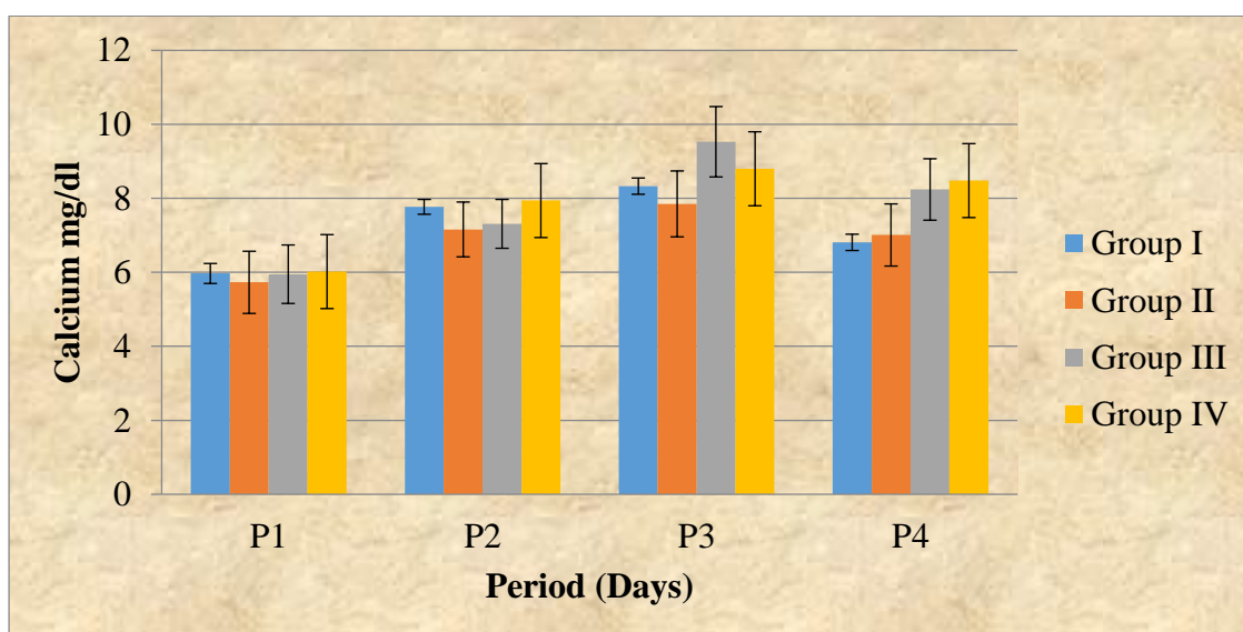
Fig. 3. Calcium levels (mg/dl) at various periods in different treatment groups
