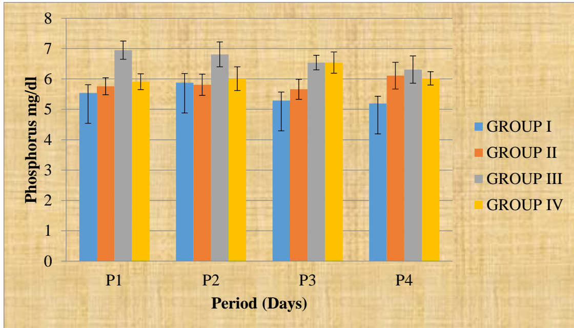
Fig. 4. Phosphorus levels (mg/dl) at various periods in different treatment groups
