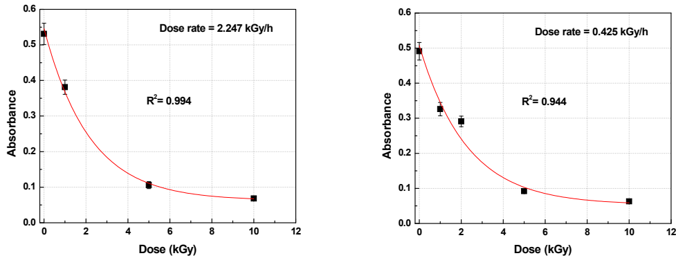
Fig. 4. Variation of absorbance of red cabbage in acidic solution A2 with irradiation dose at different dose rate 0.42513, 2.2470, 9.2585, 20.9714, 31.5389, 38.8829 kGy/h
