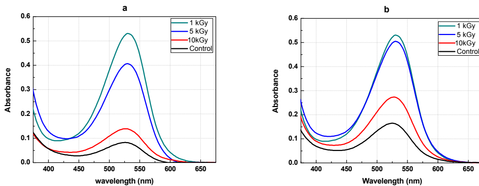
Fig. 2. Variation of absorption spectrums of red cabbage solution (pH=3.6) with respect to gamma radiation dose (from 1 to 10 kGy) at different dose rate: (a) 9.2585 kGy/h (a), 38.8829 kGy/h (b)
